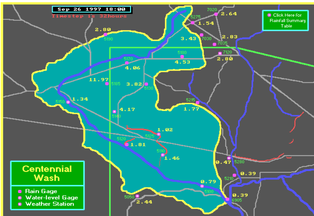
Figure 8. A graphic of Centennial Wash indicating the total amount of precipitation during the September 25 – 26, 1997 Nora event. Tiger Wash Fan gage number 5140 had a total of 4.17 inches of rain.
