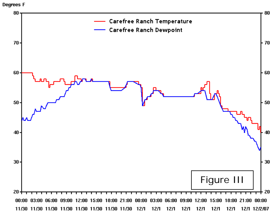
Figure III above shows a plot of temperature and dewpoint at our Carefree Ranch weather station in northeast Maricopa County - elevation 2,960 feet.
