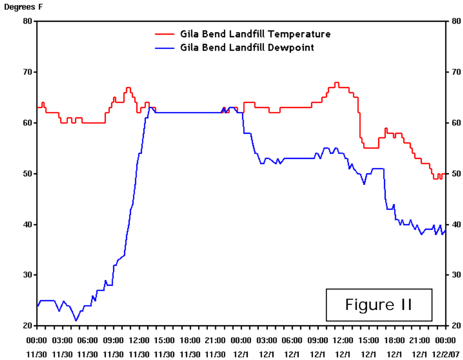
Figure II above shows a plot of temperature and dewpoint at our Gila Bend Landfill weather station in southwest Maricopa County - elevation 750 feet.
