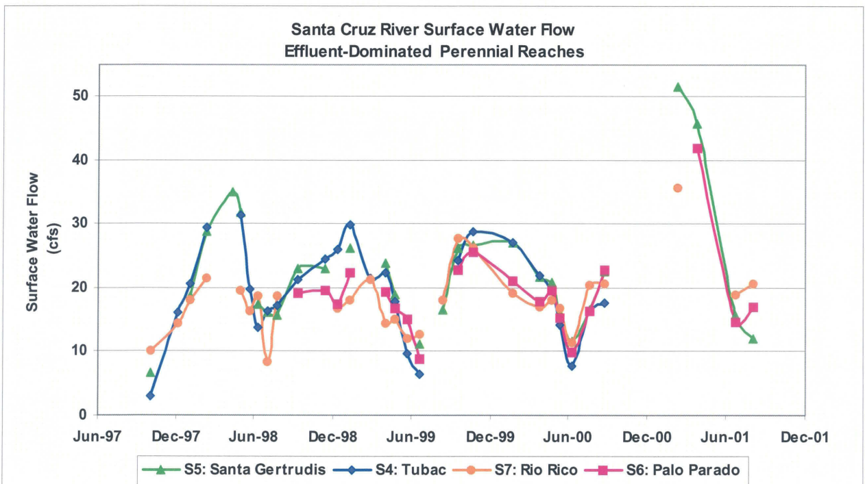
Figure 20. Surface water flow in the effluent-dominated portion of the perennial sections of the Santa Cruz River.
