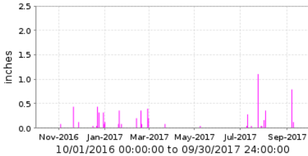
5105 Delaney Wash [WT] Period Rainfall/1 day
