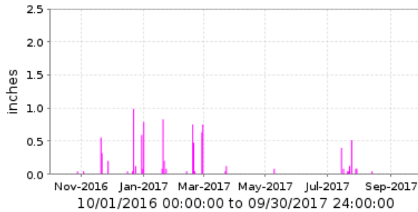
5455 Wittmann [WT] Period Rainfall/1 day
