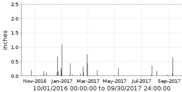
5090 Centennial Wash @ Wenden [HQ] Period Rainfall/1 day
