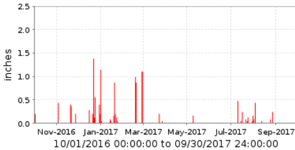
5585 Skunk Cr. near New River [WT] Period Rainfall/1 day
