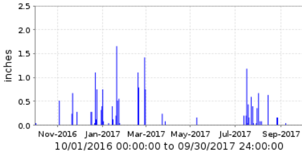
■ 4960 Seven Springs Wash [HM] Period Rainfall/1 day
