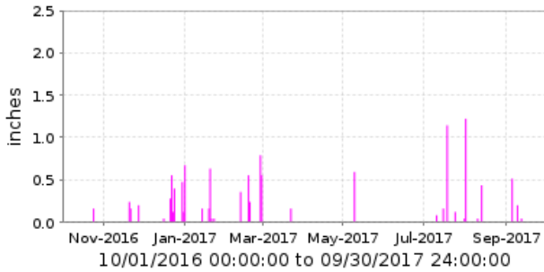
■ 5175 Centennial Wash near Aguila [YH] Period Rainfall/1 day
