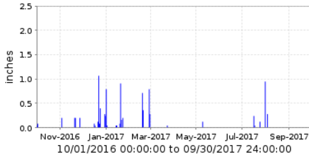
4895 Desert Hills Wash [WT] Period Rainfall/1 day
