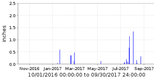
31100 Reid Park Period Rainfall/1 day
