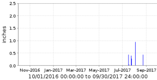
56600 El Dorado Park Period Rainfall/1 day
