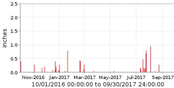
4540 Fitch Park [TP] Period Rainfall/1 day
