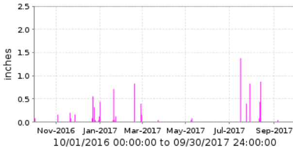
5410 Dysart Drain @ Luke AFB [WT] Period Rainfall/1 day
