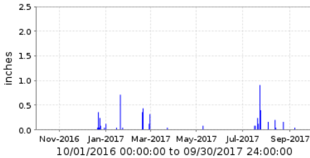
32600 Val Vista Dr. @ Pueblo Ave. Period Rainfall/1 day
