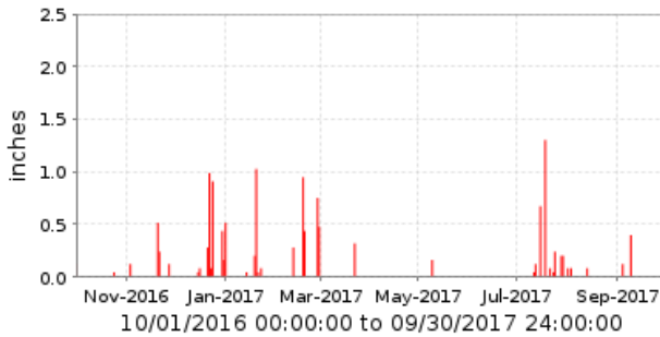
7165 Antelope Creek [YH] Period Rainfall/1 day
