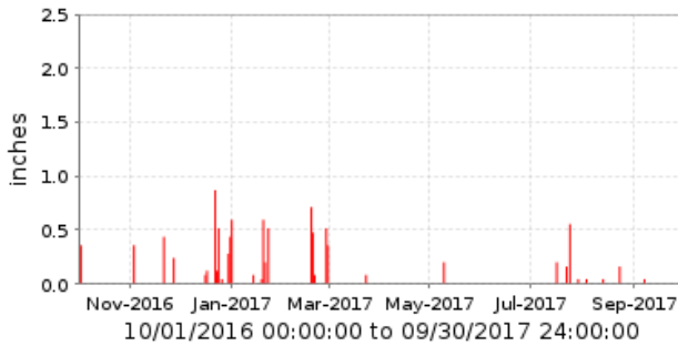
4670 Pima Rd. @ Jomax Rd. [TP] Period Rainfall/1 day
