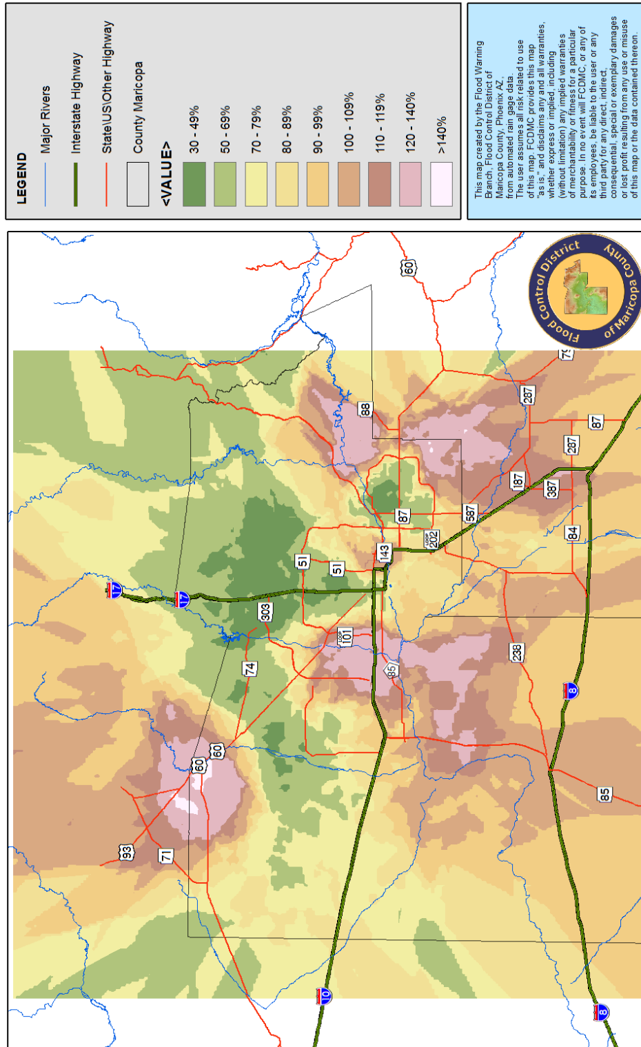
Monsoon Rainfall as % of Normal: Jun. 15 - Sep. 30, 2017
