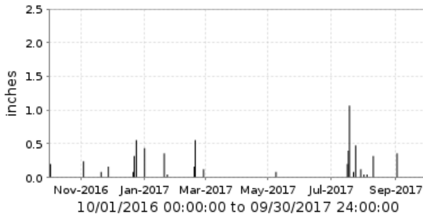
6955 Maricopa Mountains [OT] Period Rainfall/1 day
