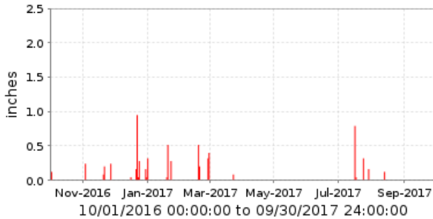
4775 Maryland Ave. @ 27th Ave. Period Rainfall/1 day
