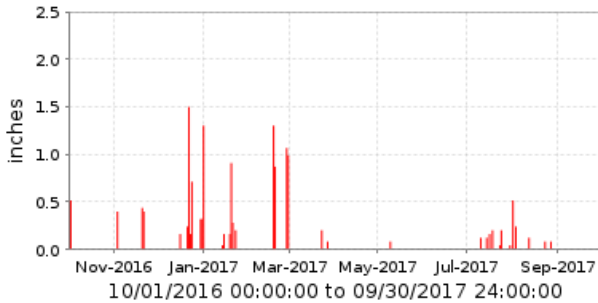
5635 New River Fire [TM] Period Rainfall/1 day
