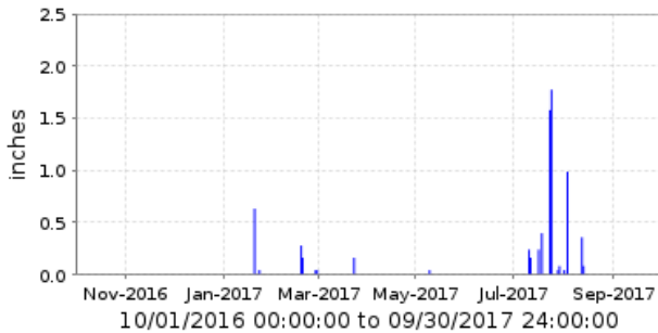
36200 Queen Creek Water Tank Period Rainfall/1 day
