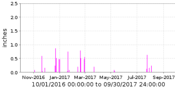
5240 Belmont Mountains [WT] Period Rainfall/1 day
