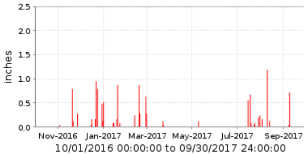
7090 Casandro Wash [YH] Period Rainfall/1 day
