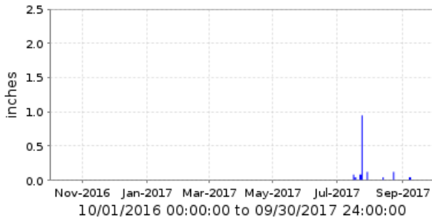
76300 Ranch Gate Road Period Rainfall/1 day
