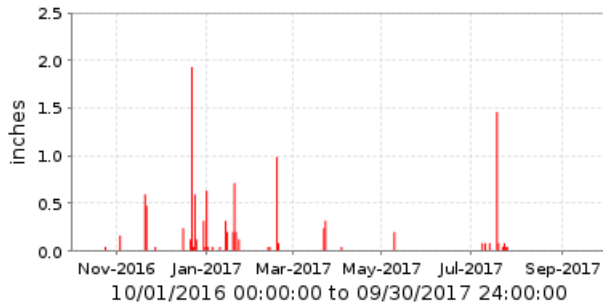
5805 Dewey [TM] Period Rainfall/1 day
