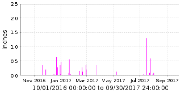
5120 Centennial Levee [BM] Period Rainfall/1 day
