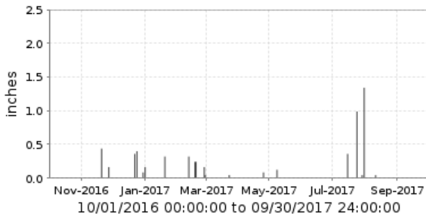
5000 Mt. Oatman [BM] Period Rainfall/1 day
