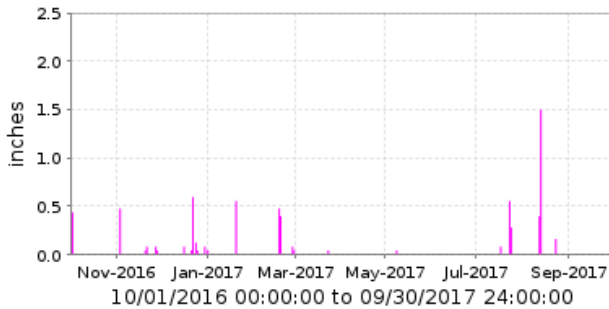
6535 Pecos Basin Period Rainfall/1 day
