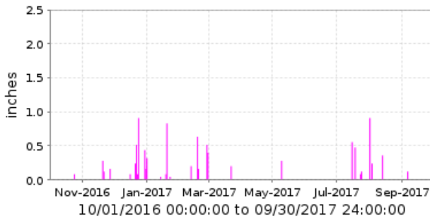
5180 Centennial Wash [YH] Period Rainfall/1 day
