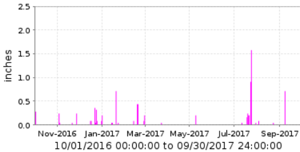
6625 Signal Butte FRS Period Rainfall/1 day
