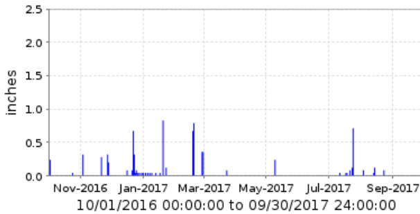
■ 5995 Hesperus Wash [TP] Period Rainfall/1 day
