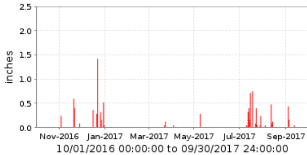
5700 Horsethief Basin Period Rainfall/1 day
