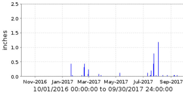
34700 Main St. @ Hawes Rd. Period Rainfall/1 day
