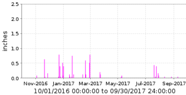
5495 Daggs Wash [WT] Period Rainfall/1 day
