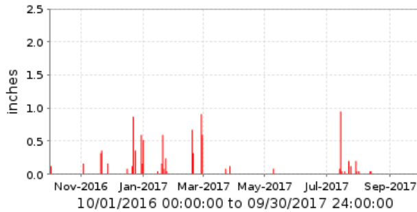
5660 Lake Pleasant North [WT] Period Rainfall/1 day
