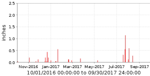
780 Gila River at Olberg [SP] Period Rainfall/1 day
