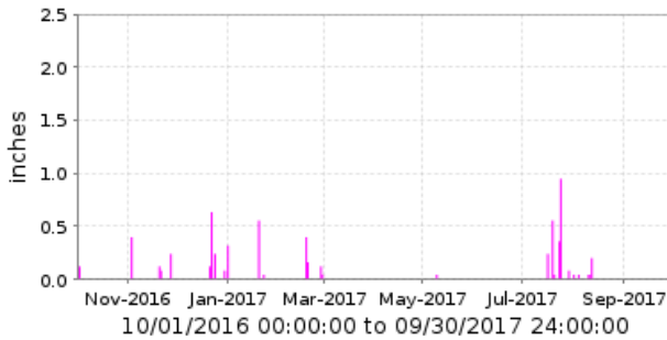
6890 Estrella Fan Period Rainfall/1 day
