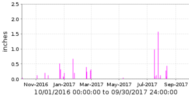
6820 White Tank FRS #4 [WT] Period Rainfall/1 day
