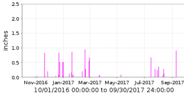
5270 Box Wash [WT] Period Rainfall/1 day
