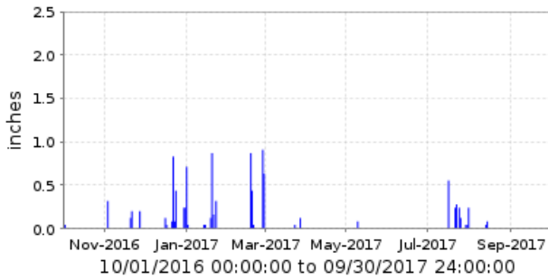
20600 Galloway Wash @ Galloway Rd. Period Rainfall/1 day
