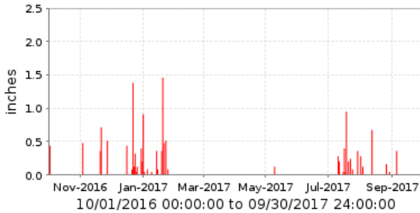
■ 5640 Cooks Mesa Period Rainfall/1 day
