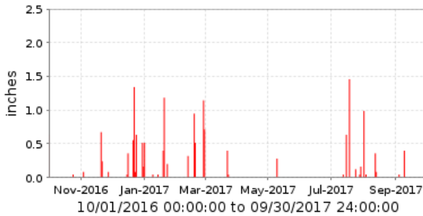
7005 Mid-Martinez Creek [YH] Period Rainfall/1 day
