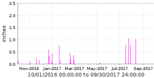
5420 Camelback Rd. @ Citrus Rd. [WT] Period Rainfall/1 day
