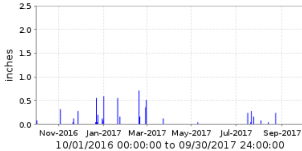
4800 Dreamy Draw Dam Period Rainfall/1 day
