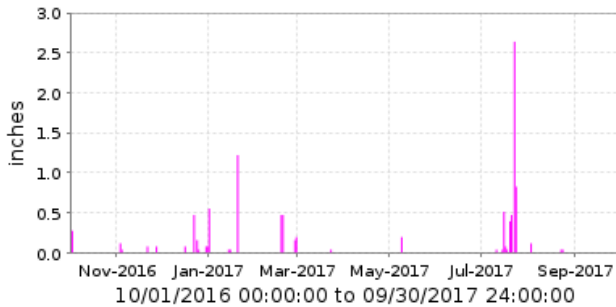
6655 Thunder Mountain Period Rainfall/1 day
