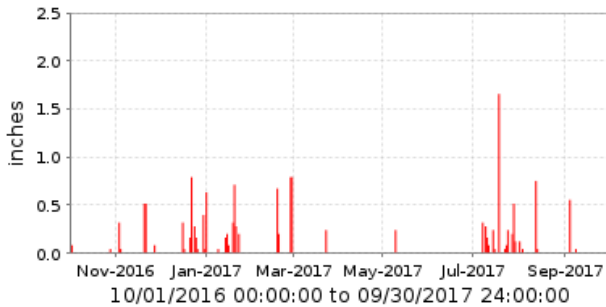
5760 Horner Mountain Ranch [TM] Period Rainfall/1 day
