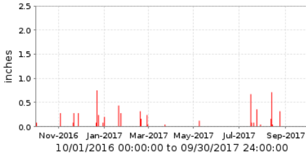
4765 Buckeye Rd. @ 75th Ave. Period Rainfall/1 day
