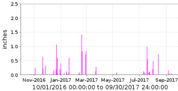
5485 Upper Trilby Wash [WT] Period Rainfall/1 day
